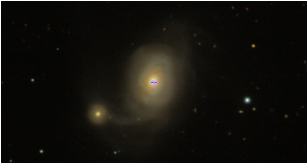
Image 6: SWIFT J2318.9+0013 (NGC 7603)
