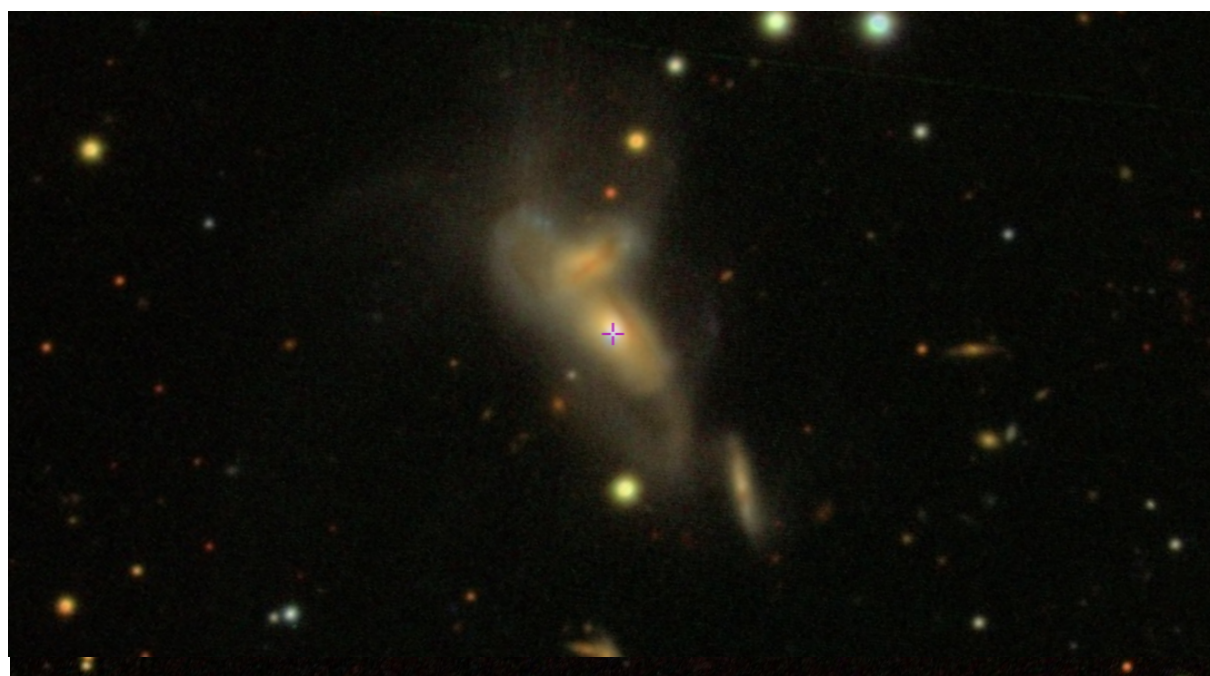
Image 4: SWIFT J2207.3+1013 (NGC 7212)
